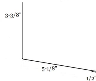
Endwall Flashing (EW1)
