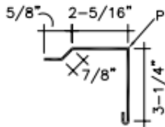
Gable Rake GR4
