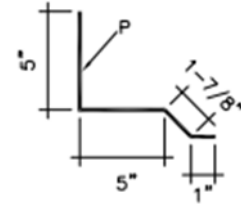
Side Wall Flashing (SW2)
