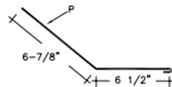
Transition Flashing (TF1)
