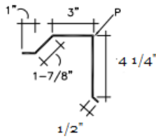
Gable Rake GR7
