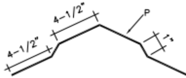
Ridge Cap RC7
