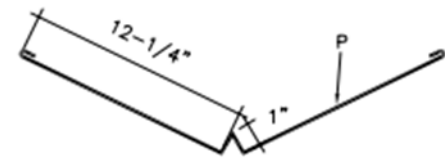
Preformed Valley (PV2)
